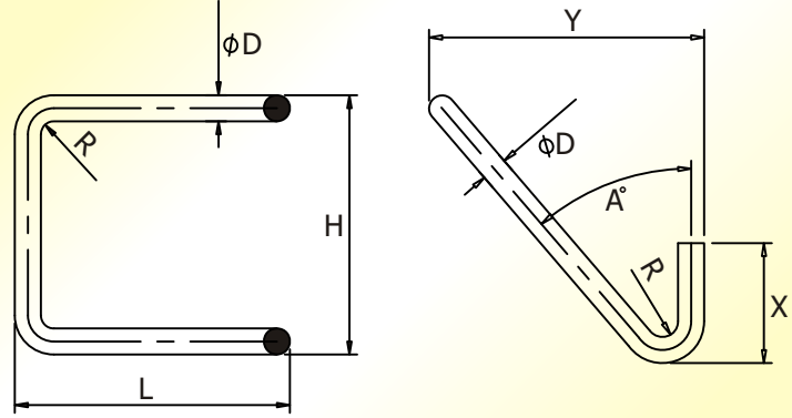
HOLDER HOOK
