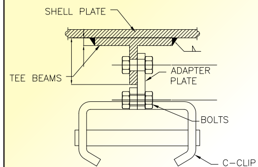
ASSEMBLY OF T-BEAM ADAPTER & C-CLIP
