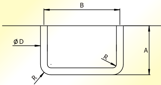
HOLDER HOOK
