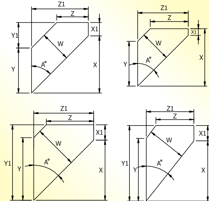
STIFFNER PLATE
