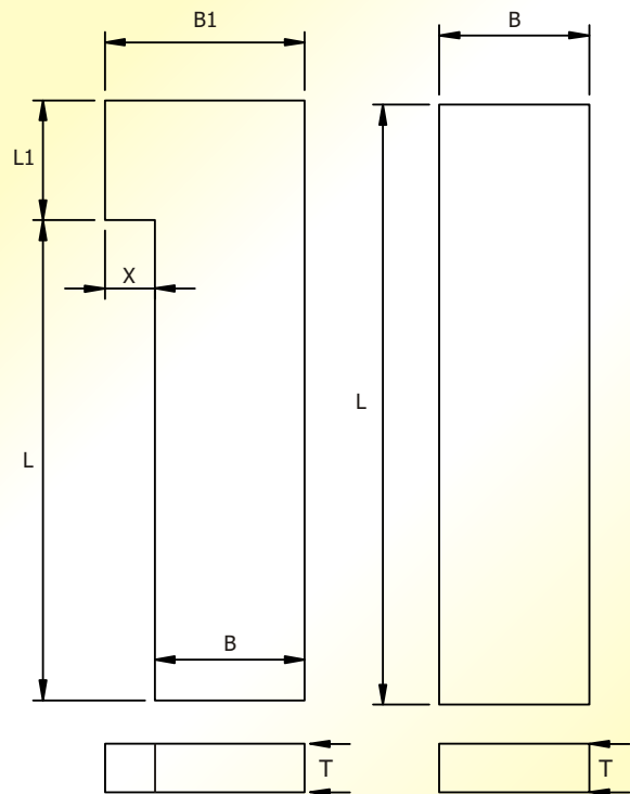
RETAINER PLATE
